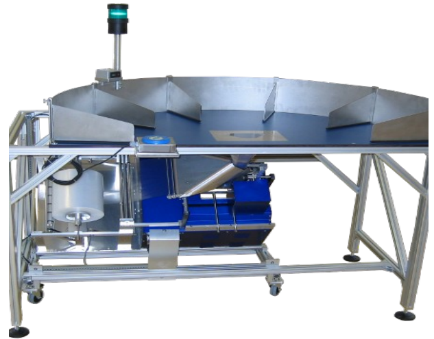
Picture 2: LBX100 sorting table with feed opening into a Lauper LVX packaging machine. (Arrangement under the table)
