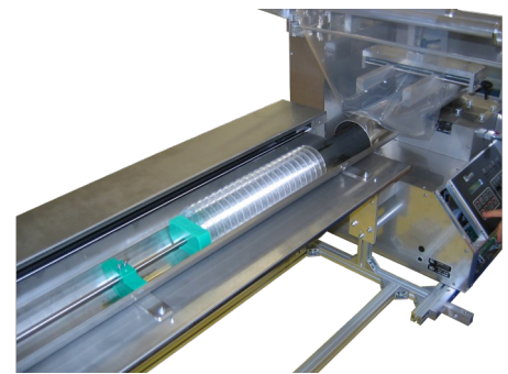
Picture 3: Example for stacked cups packaging with round slide-in channel
